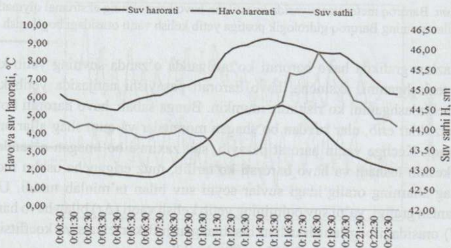
8-rasm. Barqroqsoy o'ng irmog'ining suv sathi ( H , sm ), suv harorati ( T_{suv} , ^{\circ}C ) hamda havo harorat ( T , ^{\circ}C ) larining kun ichida tebranishi.
